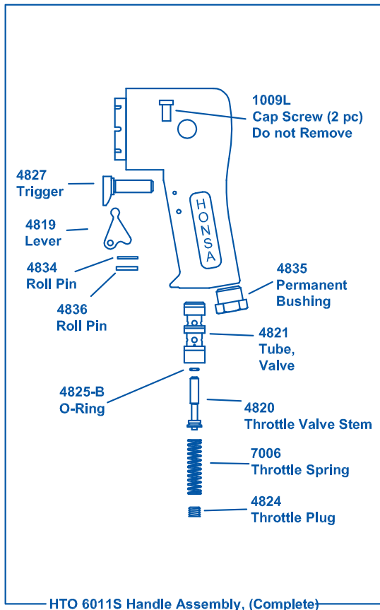
HTO 6011S Handle Assembly, (Complete)
