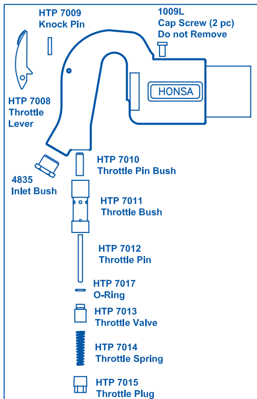
B1700 Handle Assembly, (Complete)
